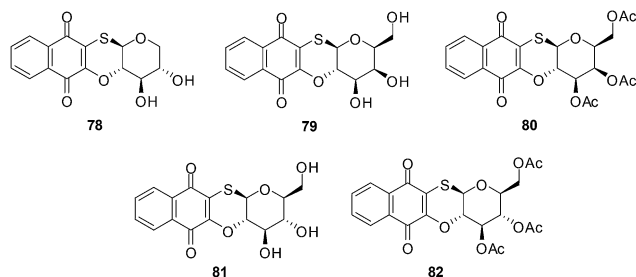
Fig. 22 S -glycosides of 1,4-naphthoquinones highly active against leukemia (HL-60) cells.
