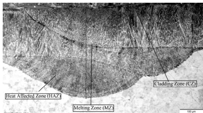
Fig. 3. Microstructure of sample 1 showing the different zones
