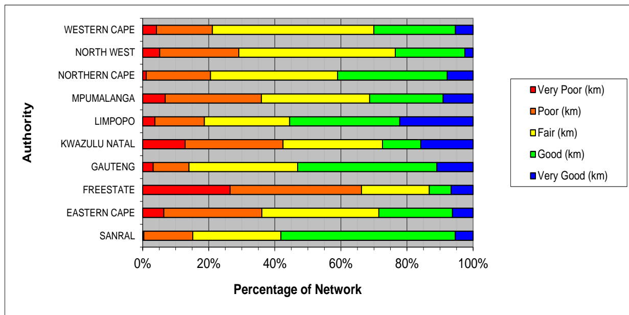
Figure 2: Summary of South African Road Network Condition (Source: SANRAL).
