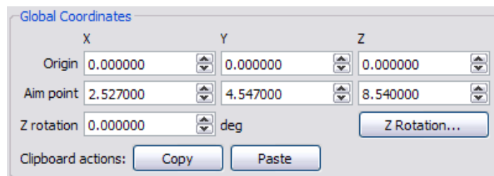
Figure 6. Screenshot shows the heliostat aiming point within the global coordinate system
