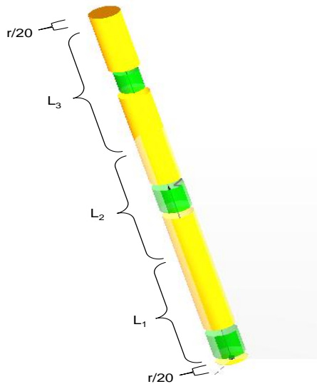
Fig.3: monopole antenna with three RLC loading.
