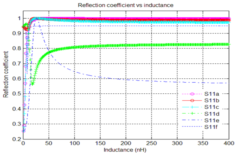
Fig.2: Reflection coefficient resulting from Inductance range conducted on three different locations on a monopole
