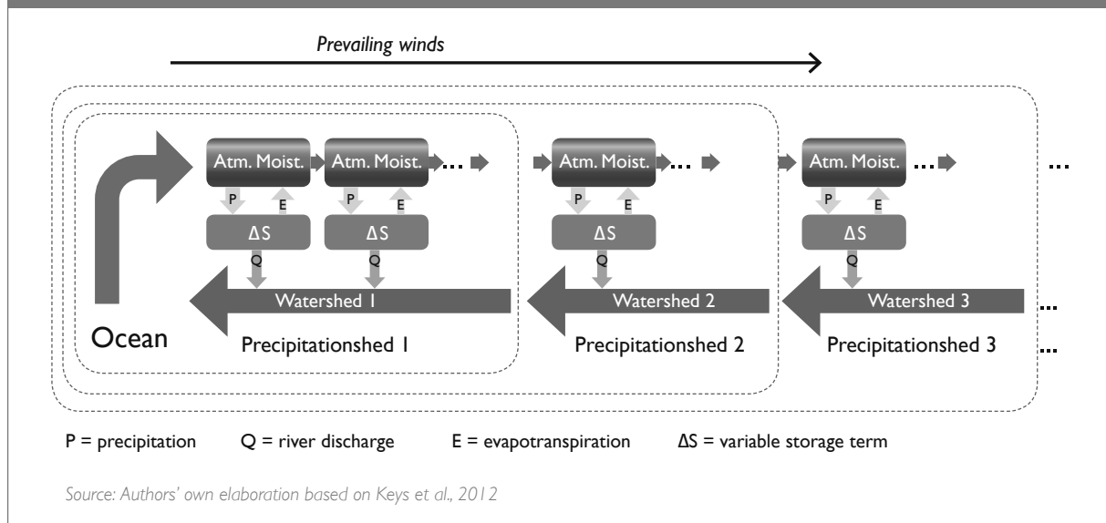
Conceptual model of the water balance along a series of spatial units following the prevailing winds from an ocean-land interface
