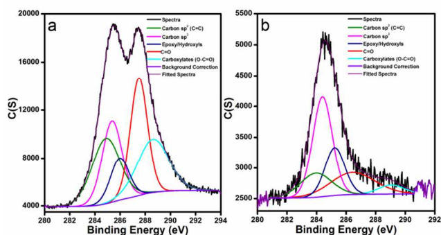
Fig. 5 Fitted XPS C1s spectra of (a) as-prepared GO sample and (b) spray pyrolyzed sample at 600^\circ\text{C} .
