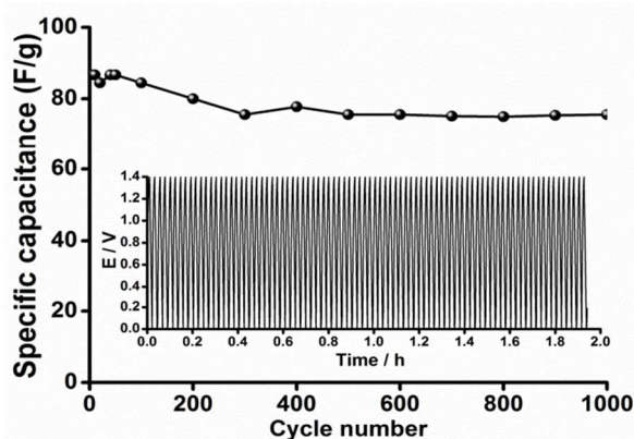
Figure 8. Cycle life of the assembled asymmetric supercapacitor device tested over 1000 cycles at a current density of 0.2 \text{ Ag}^{-1} within a potential window of 1.4 V.
