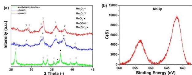
Fig. 2 (a) XRD patterns of the manganese based composite showing the different phases present in the Mn Oxides/Hydroxides and the rGOMO materials spray pyrolyzed at 600°C. (b) XPS spectrum of rGOMO1 sample in the Mn region.
