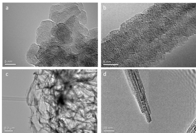
Fig. 4 HRTEM micrographs of Manganese oxide-hydroxide showing (a) an agglomeration of nanoparticles which results in nanorods as shown in (b). The combination of rGO and \text{Mn}_2\text{O}_3/\text{Mn}_3\text{O}_4 (c) and a high magnification, (d) rGOMO1.
