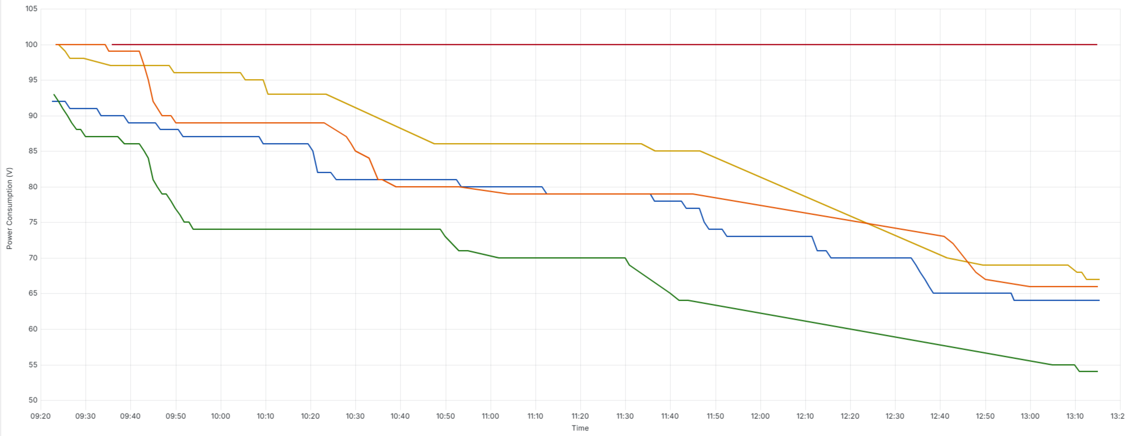
Power Consumption of LoRa Devices During Sea Communications Test (Calm Weather Conditions)
