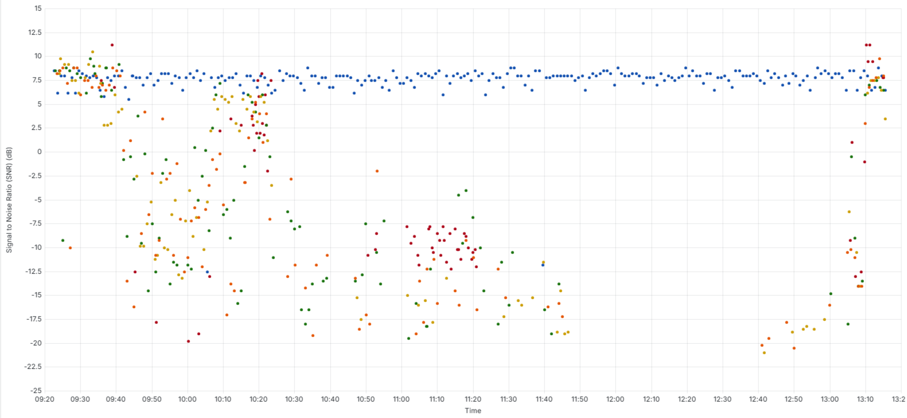
Signal to Noise Ratio (SNR) of LoRa Devices During Sea Communications Test (Calm Weather Conditions)
