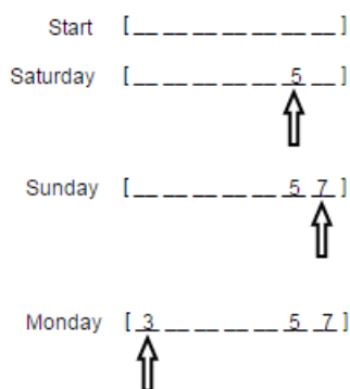
Figure 1: Aggregating data into a rolling array
