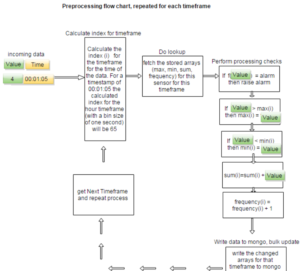
Figure 4: Processing the data
