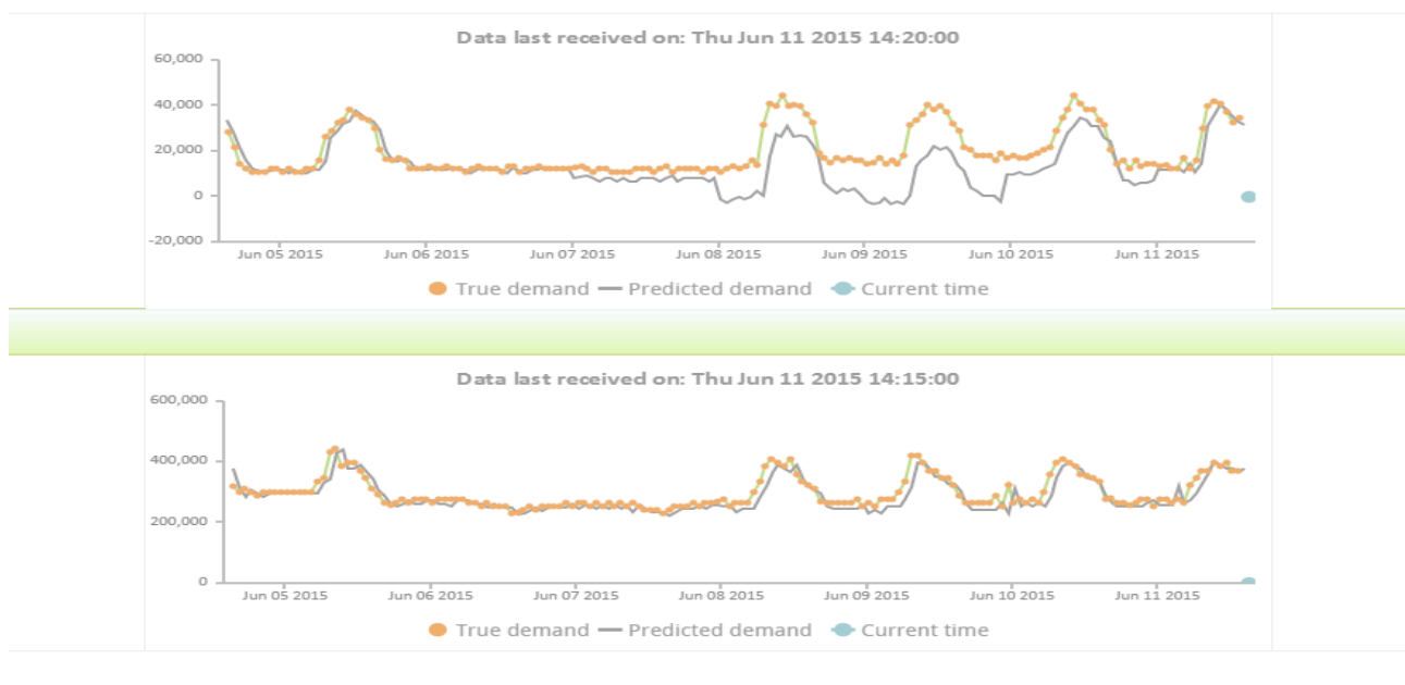
Figure 7: The ONE WEEK time-frame
