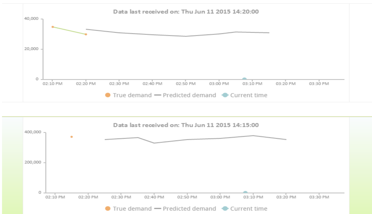
Figure 5: The ONE HOUR time-frame for 2 different sensors
