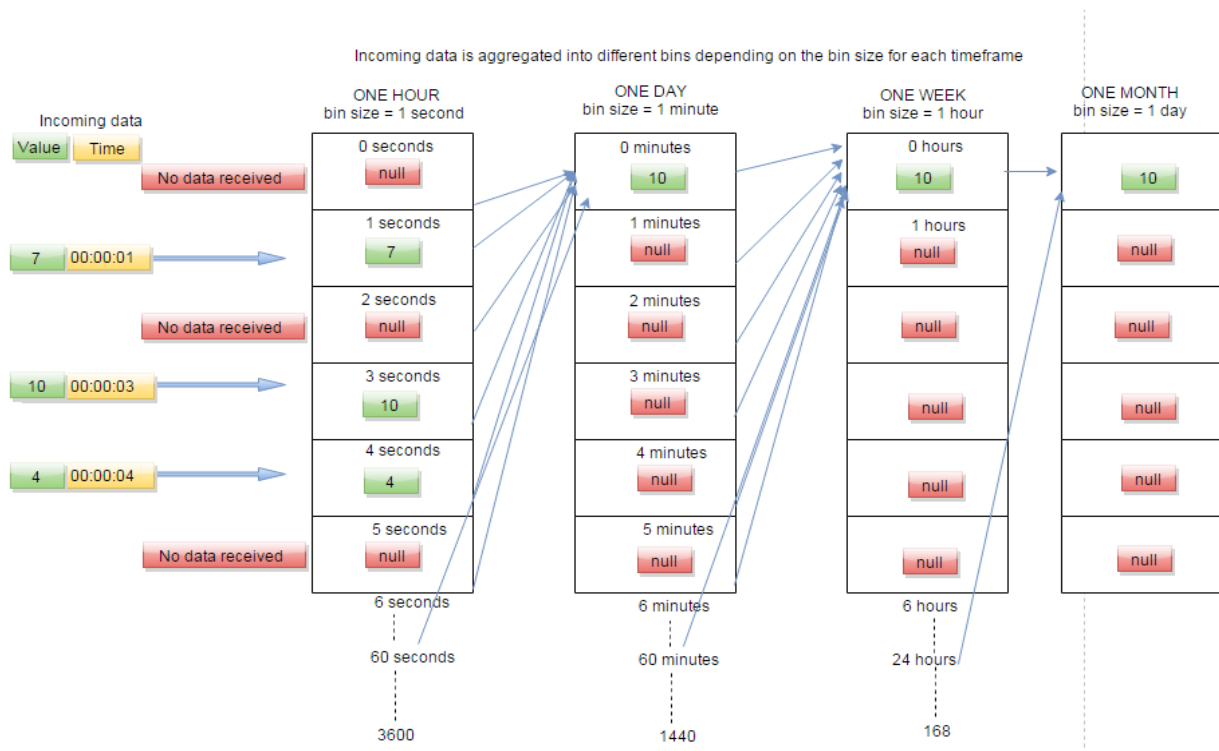
Figure 2: Aggregating data into different rolling time-frame arrays.
