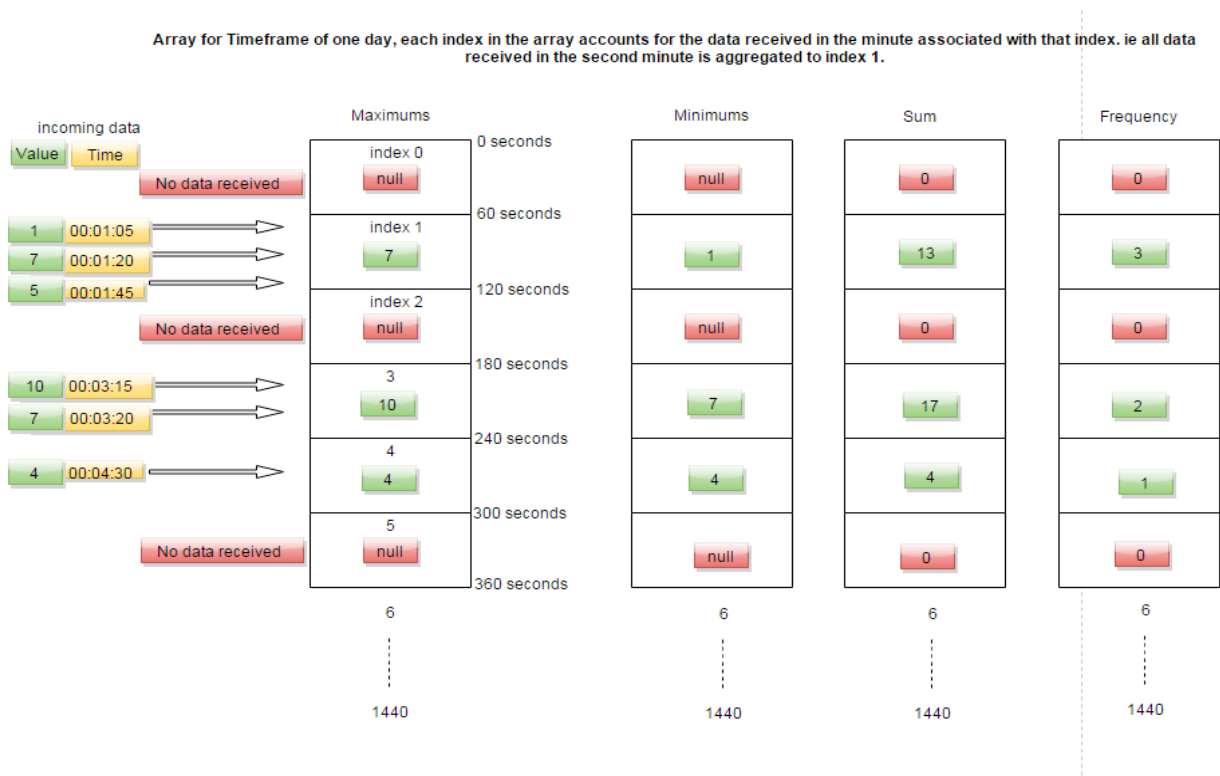
Figure 3: The data format per time-frame.
