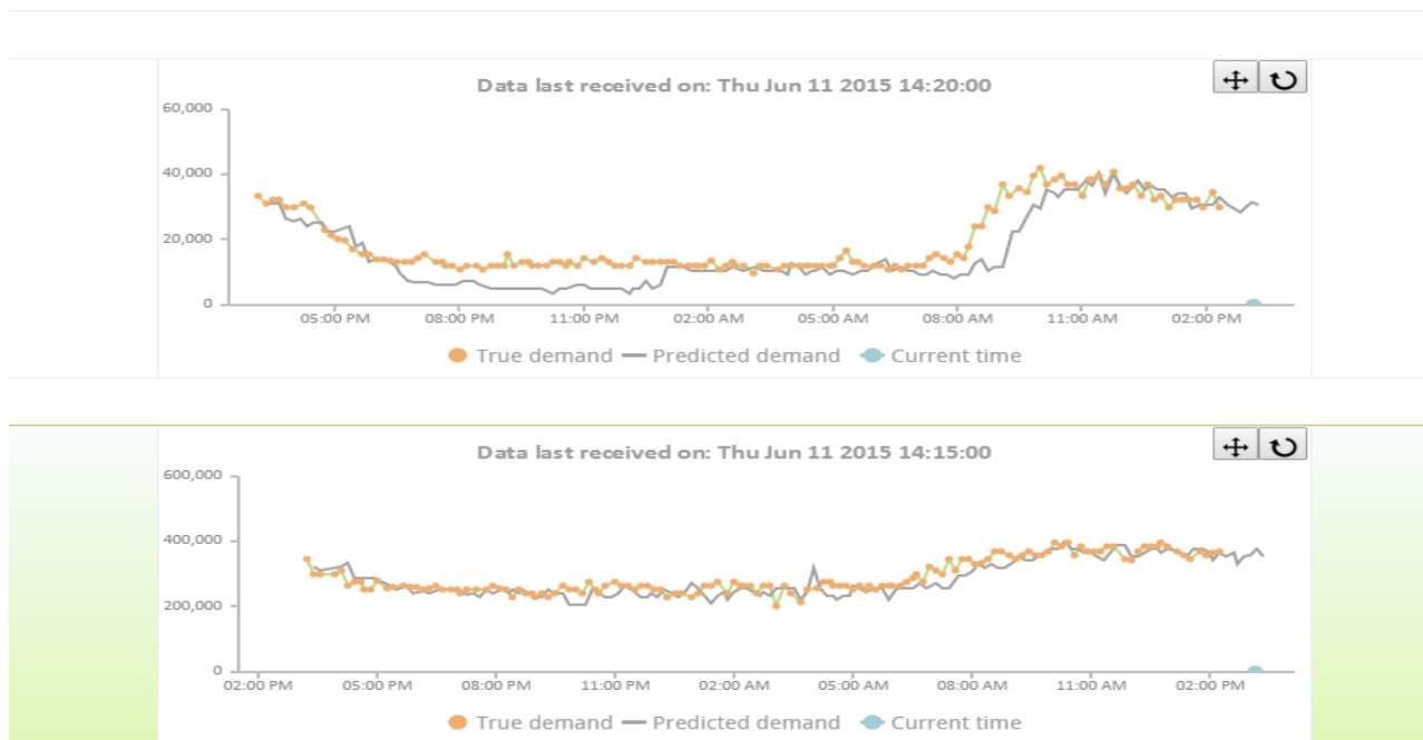
Figure 6: The ONE DAY time-frame
