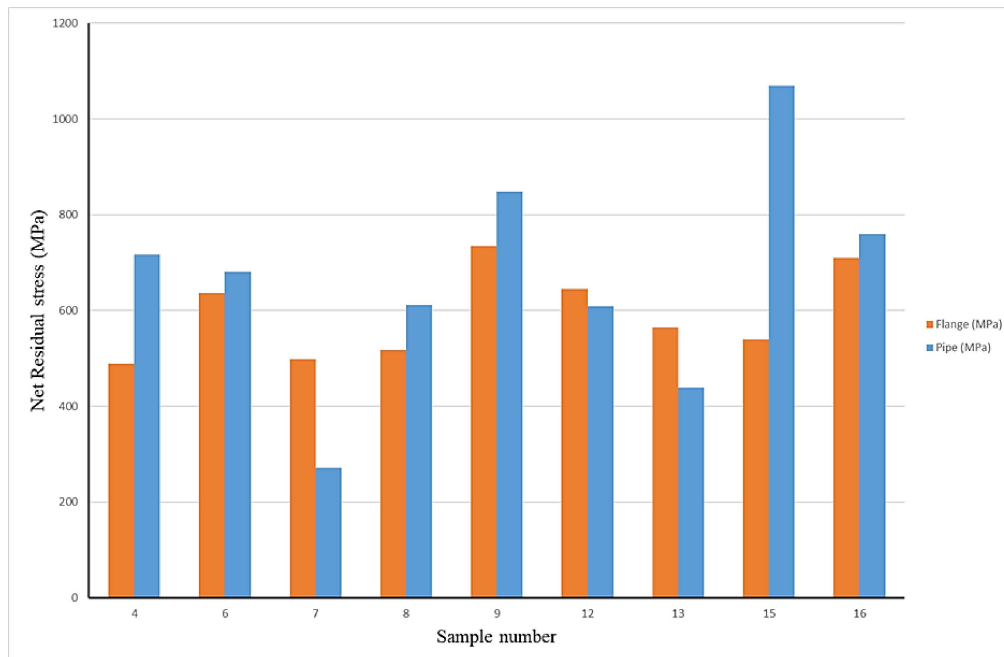
Figure 4. A bar graph of the net welding residual stress measured in the pipe and the plate (flange)
