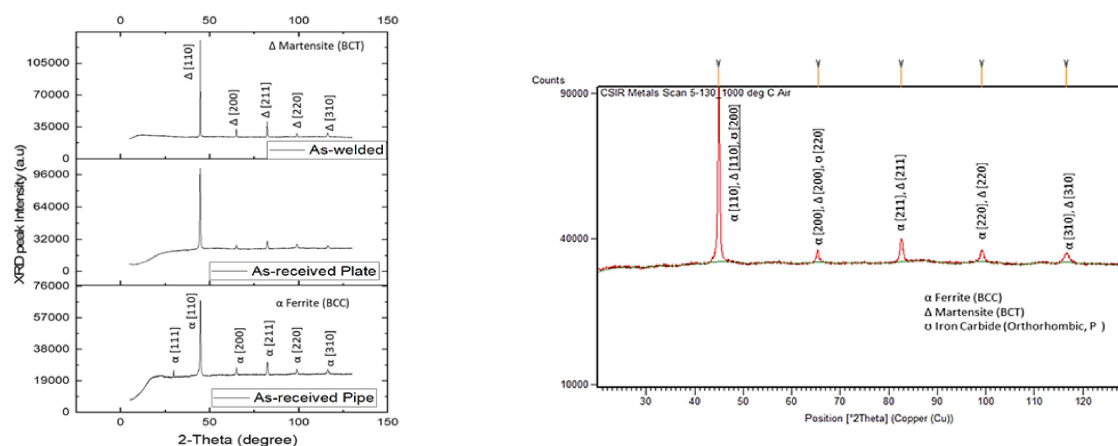
Figure 7. XRD scans of the test specimens as-received of the plate, as-received of the pipe, and the XRD plot of the heat-treated specimen and air-cooled.
