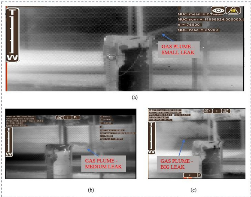
Fig. 10. Sulphur hexafluoride leak detection (a) small leak (b) medium (c) big leak.
