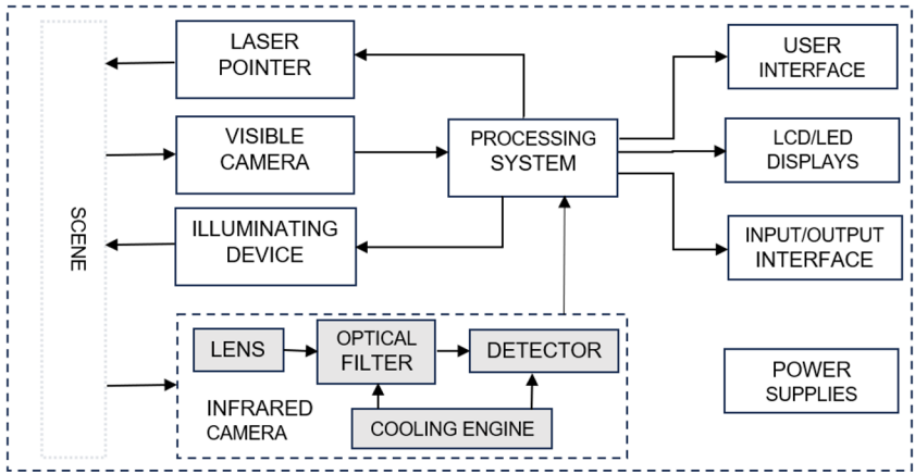
Fig. 3. Overview of the optical gas imaging system.
