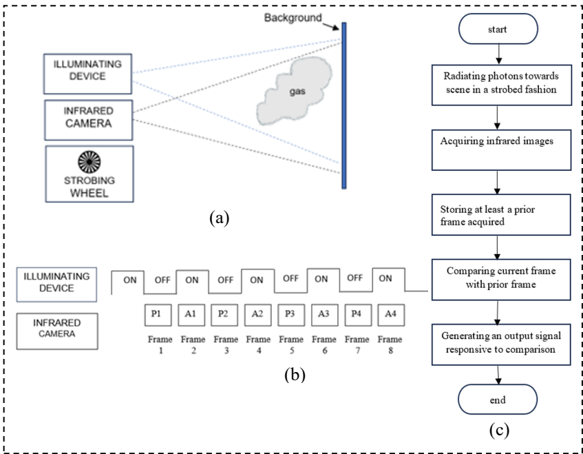
Fig. 2. Illustrating strobed illumination [11] (a) the concept (c) the mechanism (c) the flowchart.
