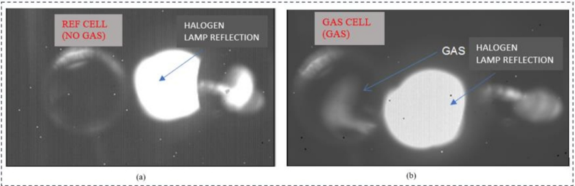
Fig. 7. Effect of halogen lamp strobed illumination on gas visibility (a) reference cell (b) gas cell.
