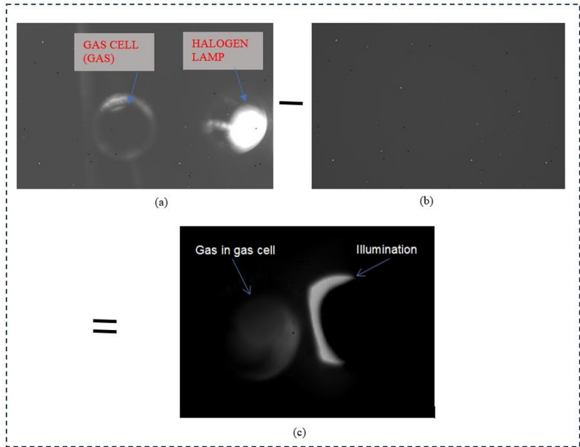
Fig. 8. Effect of continuous illumination on gas visibility (a) illumination on (b) illumination off (c) illuminated gas.
