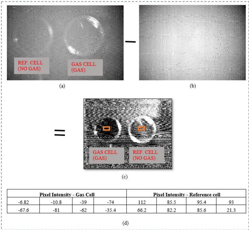
Fig. 6. Illustration of the laser strobing effect on gas visibility (a) laser strobing (b) no strobing (c) subtraction of (a) and (b) (d) pixel intensity values.
