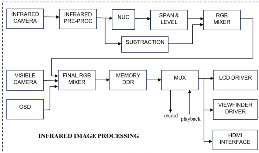
Fig. 4. Infrared image processing block diagram.
