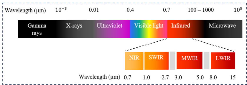
Fig.1. Position of the infrared band in the electromagnetic spectrum.
