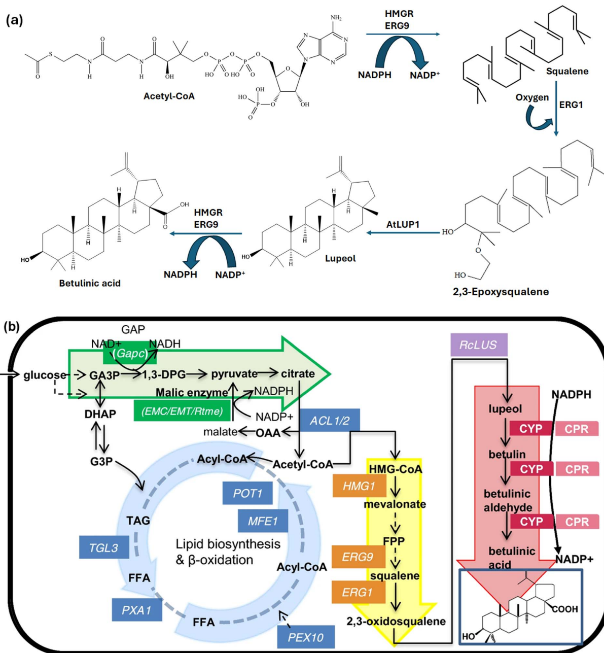
Fig. 7 (a). Reaction scheme showing the biosynthetic pathway of BA using engineered yeast S. cerevisiae . (b). Overview of the multimodular strategy for producing BA-related triterpenoids in Y. lipolytica . The BA biosynthesis pathway is divided into four modules: the red arrow indicates the heterologous CYP/CPR module (CYP-lupeol C-28 oxidase, CPR-CPR-NADPH-cytochrome P450 reductase). The yellow arrow shows the MVA module, which includes three genes (ERG1, ERG9, and HMG1). The green arrow depicts the redox cofactor supply module, featuring four introduced genes (EMC, EMT, and Rtme – encoding malic enzyme, responsible for NADPH generation, and Gapc – encoding glyceraldehyde-3-phosphate dehydrogenase, responsible for NADH production). The blue arrow represents the acetyl-CoA generation module, with seven endogenous genes overexpressed (ACL1 and ACL2, encoding ATP citrate lyase, to increase acetyl-CoA levels directly; PXA1, MFE1, PEX10, POT1, and TGL3, which participate in the \beta -oxidation pathway and are responsible for fatty acid catabolism to produce acetyl-CoA). This figure has been reproduced from ref. 57. Copyright: 2019 by the authors. This article is an open access article distributed under the terms and conditions of the Creative Commons Attribution (CC BY) license ( https://creativecommons.org/licenses/by/4.0/ ).
