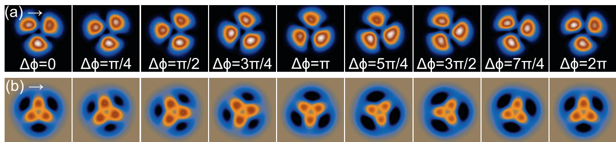
Figure 5. Rotation of the beam intensity (a) and of the OAM density (b) of the superposition \text{LG}_{0,1} + \text{LG}_{0,-2} e^{i\Delta\phi} while changing the intermodal phase difference \Delta\phi = 0 \dots 2\pi yielding a rotation of 120^\circ . Rotation in full resolution, see movie 1 in the supplementary data (available from stacks.iop.org/NJP/15/073025/mmedia ).
