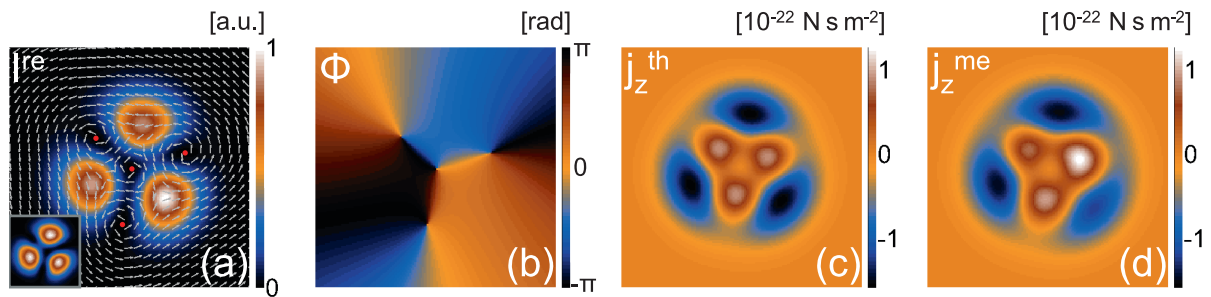
Figure 4. Characterization of a Laguerre–Gaussian beam \text{LG}_{0,1} + \text{LG}_{0,-2} e^{-i\pi/3} . (a) Reconstructed intensity and transverse Poynting vectors (red dots mark the position of the phase singularities). (b) Reconstructed phase. (c) Theoretical OAM density. (d) Measured OAM density. OAM densities in \text{N s m}^{-2} . The inset in (a) depicts the measured beam intensity.
