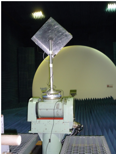
Figure 2. Set up for measuring elevation pattern of the antenna during the radiation pattern measurements performed at the anechoic chamber of the University of Pretoria
