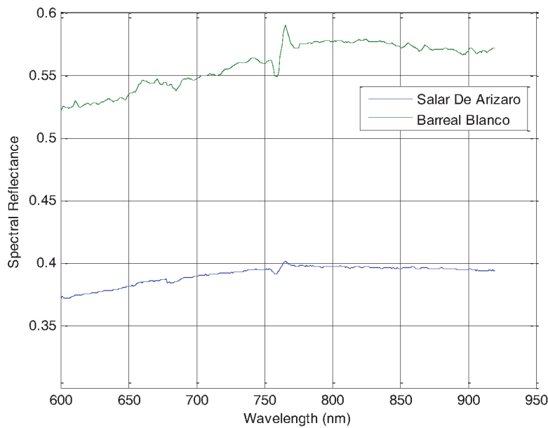
Figure 1. Surface Spectral Reflectance of Salar de Arizaro and Barreal Blanco.
