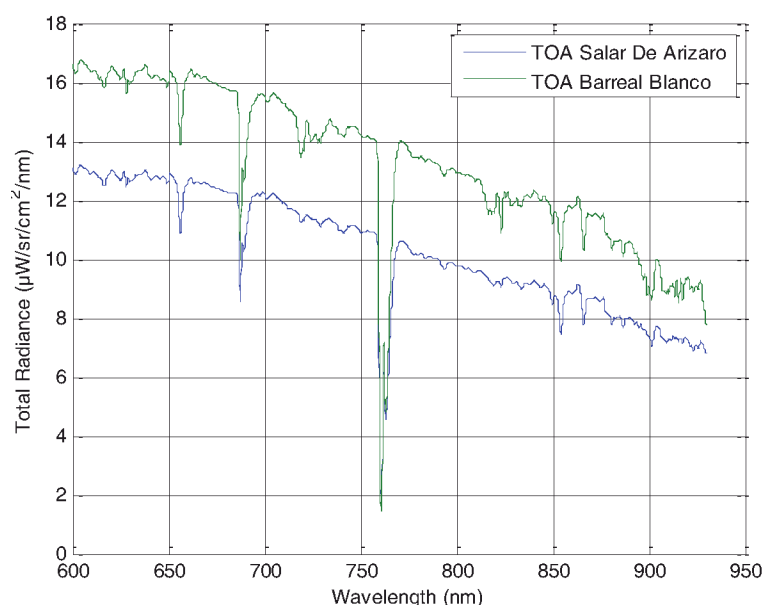
Figure 2. Top of Atmosphere Radiance for Salar De Arizaro and Barreal Blanco.
