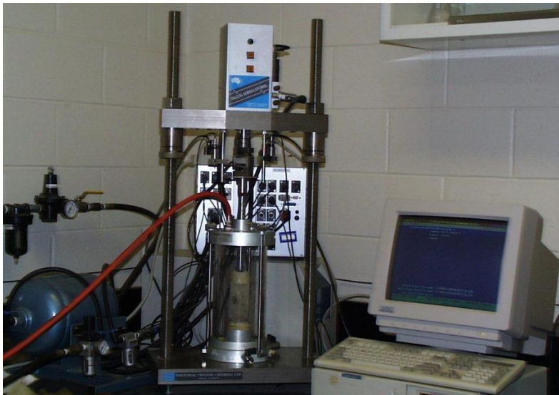
Fig. 1. Triaxial test setup for monotonic loading of the soil specimen
