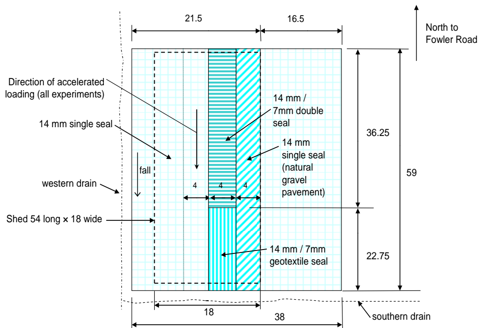
FIGURE 3 Layout of test pavements (all dimensions in meters).
