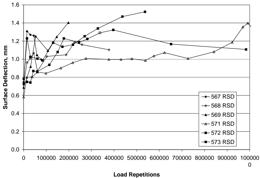
FIGURE 5 RSD surface deflections on Phase I HVS test sections.
