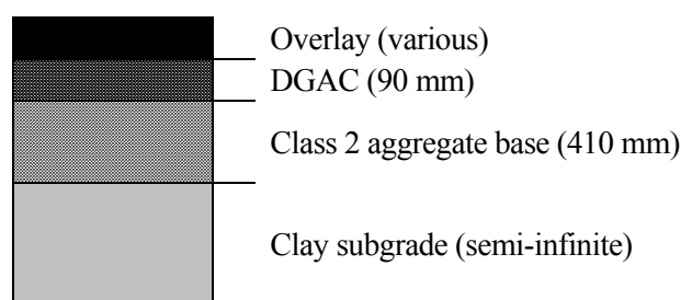
FIGURE 3 Pavement design for test road.
