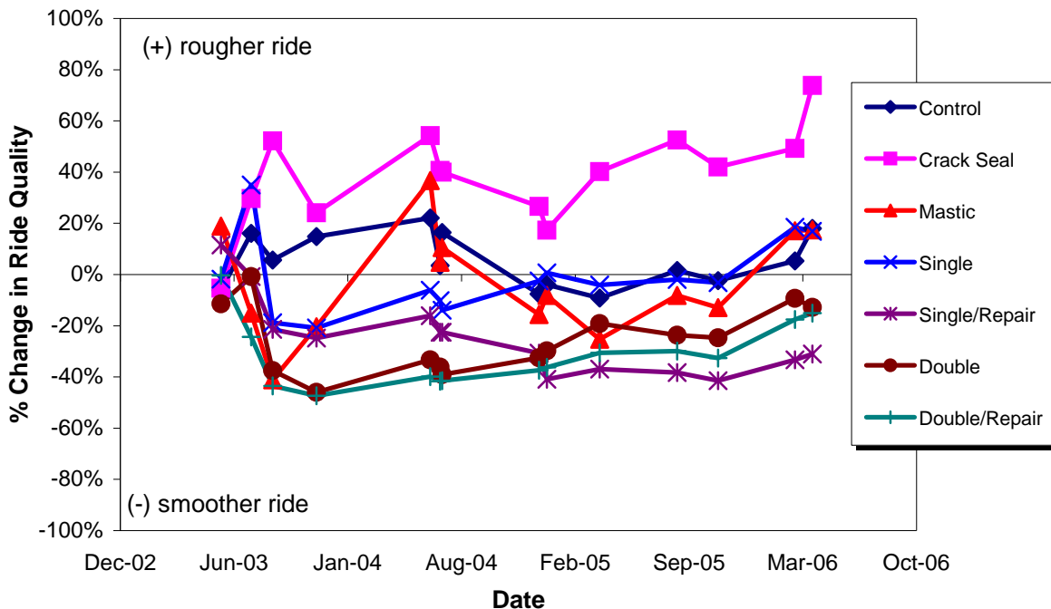
FIGURE 6 Change in ride quality since maintenance activities.
