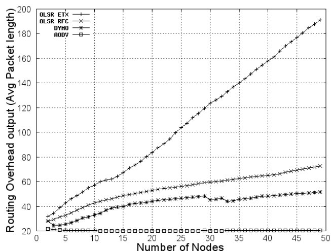
Fig. 21. Average Routing Packet length growth versus increasing number of nodes
