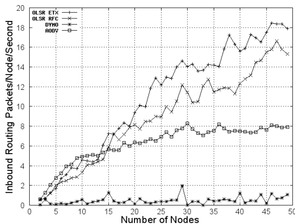
Fig. 17. Inbound routing packets per node per second versus increasing number of nodes using a growing spiral
