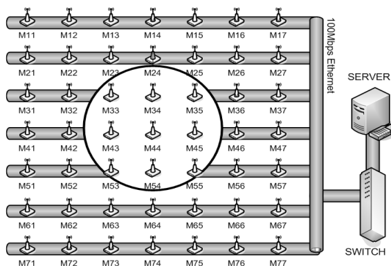
Fig. 8. The architecture of the mesh lab. Ethernet is used as a back channel to connect all the nodes to a central server through a switch. Each node is also equipped with an 802.11 network interface card.
