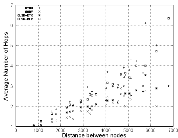
Fig. 18. Average number of hops versus distance for full 7x7 grid between all 2352 possible pairs
