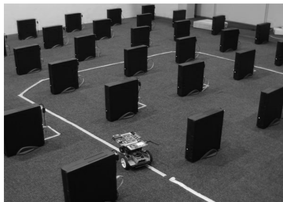
Fig. 6. Layout of the 7 by 7 grid of WiFi enabled computers, the line following robot is an option which will be explored in the future to test mobility in a mesh network.
