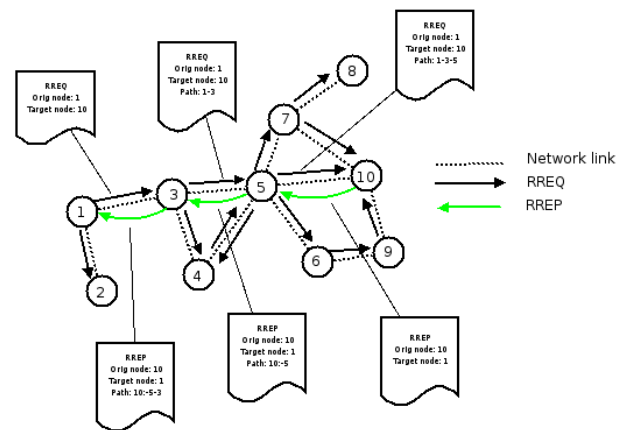
Fig. 3. DYMO routing protocol showing how path accumulation is used during route discovery
