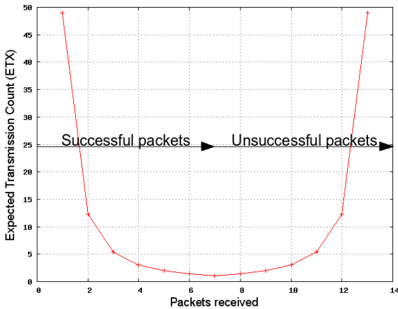
Fig. 4: ETX Path metric values for successive successful and unsuccessful packets
