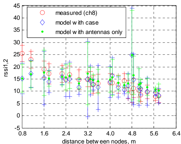
Fig. 10. Received signal strength indicator (rssi) value versus distance between nodes - measured and simulated results for a rectangular 7x7 test-bed. Crosses define the standard deviation-based range of rssi with respect to mean values shown with circles, diamonds and dots.
