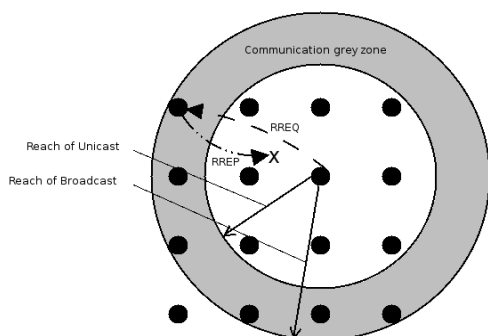
Fig. 11. Communication gray zones
