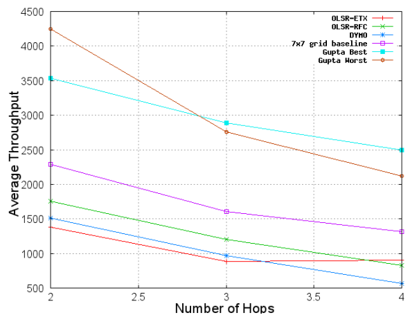
Fig. 25. Throughput performance of routing protocols against theoretical and baseline measurements
