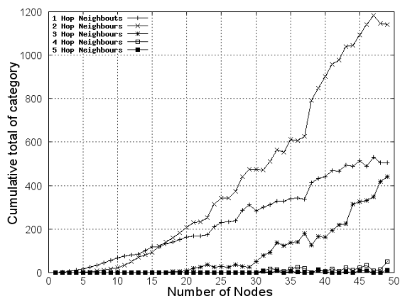
Fig. 19. Total number of links with a specific total number of hops increasing as the number of nodes increases
