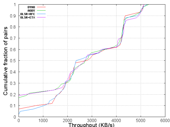
Fig. 22. Throughput CDF for 7 node string of pearls
