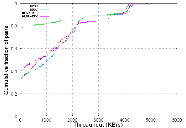
Fig. 24. Throughput CDF for 7x7 grid
