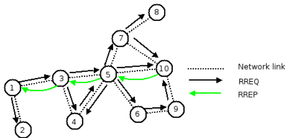
Fig. 5. AODV routing protocol showing the route discovery process
