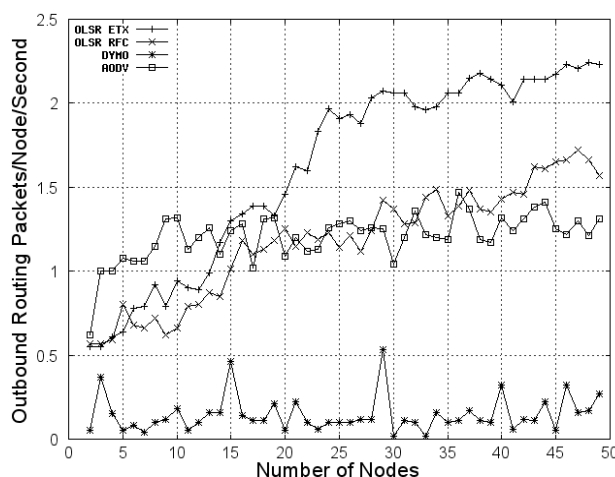
Fig. 20. Outbound routing packets per node per second versus increasing number of nodes using a growing spiral
