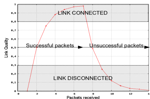
Fig. 2. Link Hysteresis in the OLSR routing protocol
