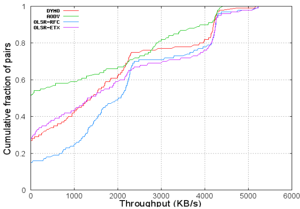
Fig. 23. Throughput CDF for 3 adjacent 7 node columns
