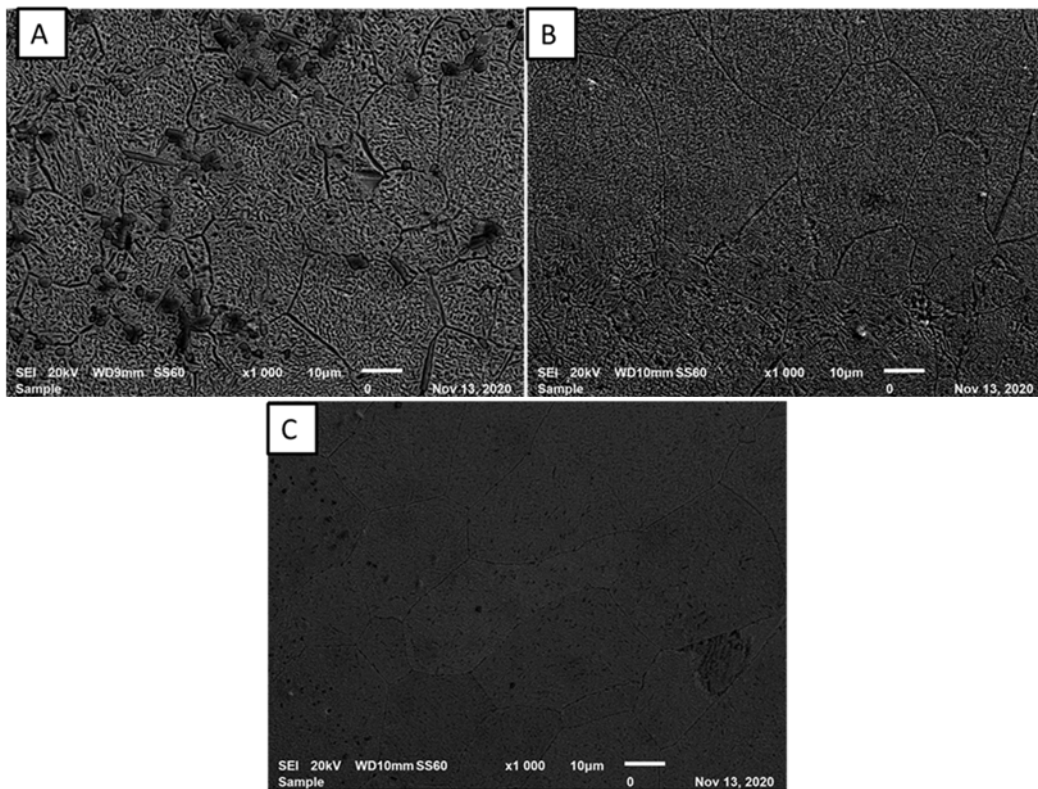
Figure 1. SEM images of Ti-Al-xNb synthesized at different Nb feed rate (A) A; (B) A1; (C) A3 and 1 L/min Nb gas carrier.
