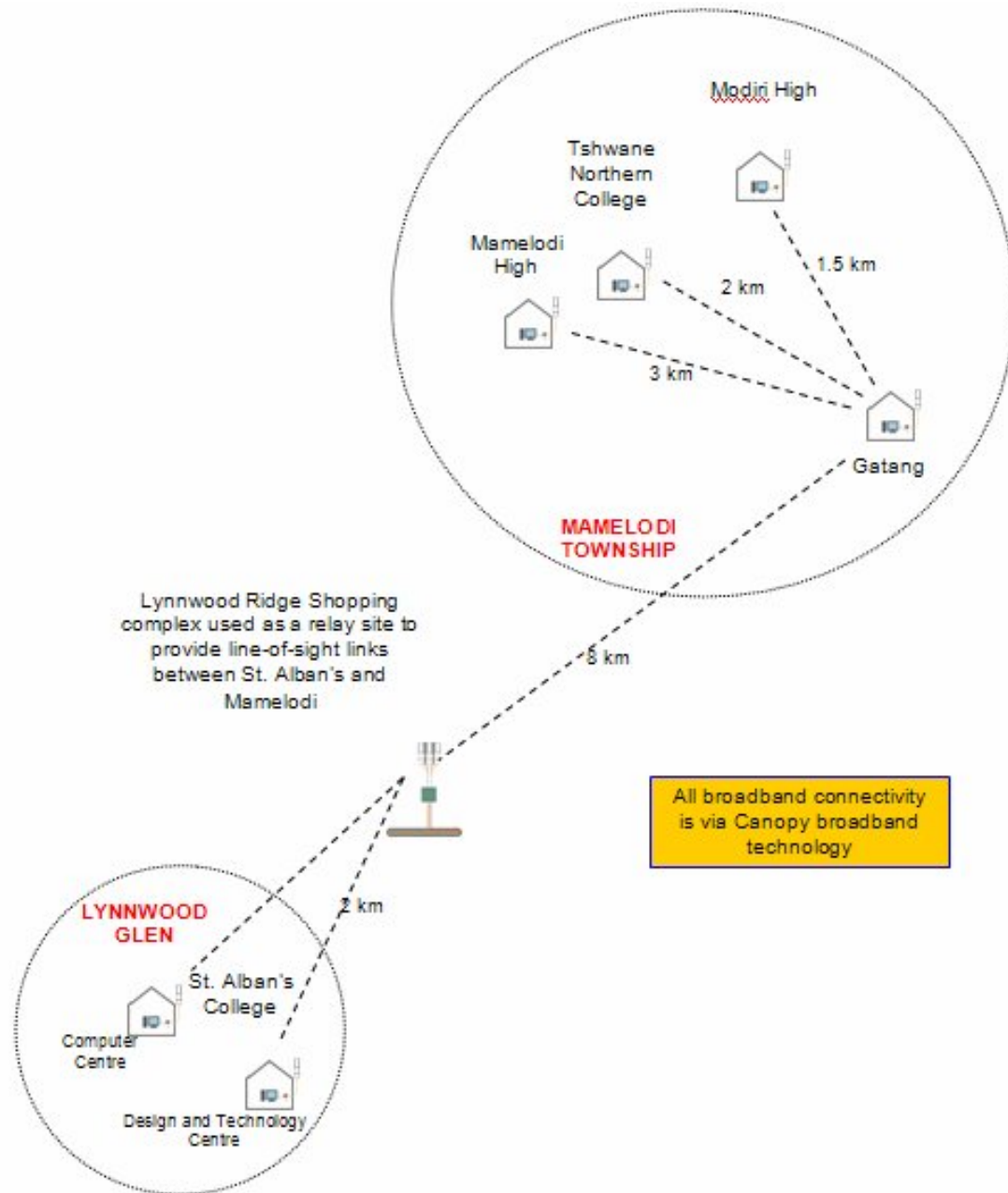
Figure 1: A schematic representation of the Ulwazi Network Diagram
