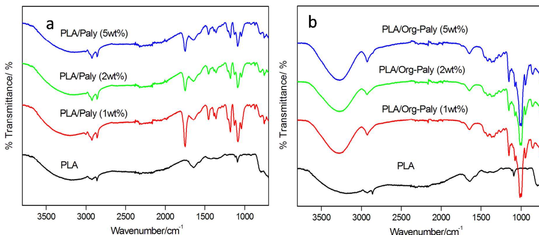
Figure 9 Fourier-transform infrared spectra of (a) PLA and PLA/Paly composites (b) PLA and PLA/Org-Paly composites
