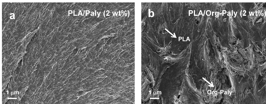
Figure 4 Field-emission scanning electron microscopy fractured-surface image of (a) PLA/Paly (2 wt.%) and (b) PLA/Org-Paly (2 wt.%) composite films.
