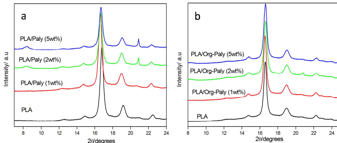
Figure 8 X-ray diffraction patterns of (a) PLA and PLA/Paly composites (b) PLA and PLA/Org-Paly composites
