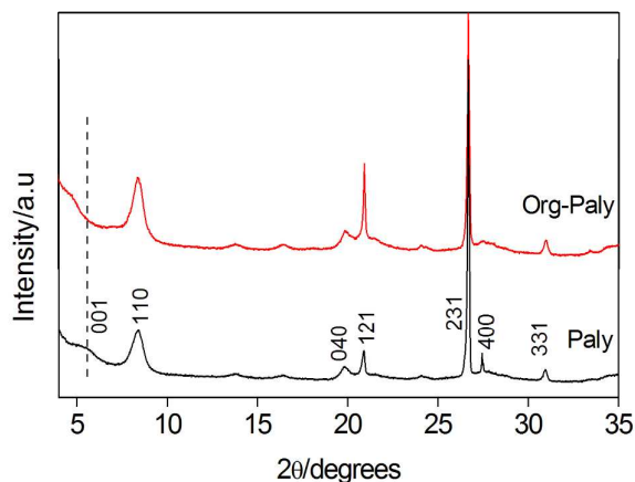
Figure 3 XRD spectra of unmodified (Paly) and of organically modified Palygorskite (Org-Paly).
