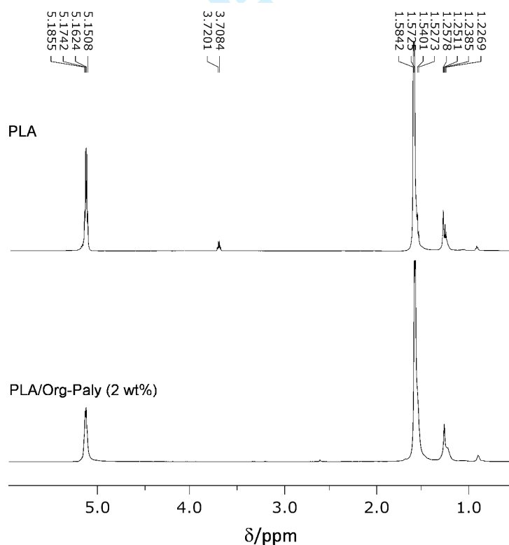
Figure 6 ^1\text{H} NMR spectra of (a) neat PLA and (b) PLA/Org-Paly (2 wt%) composites
