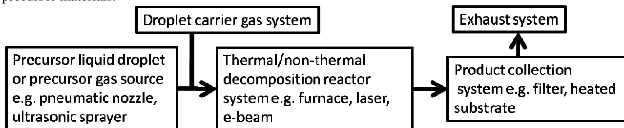
Fig. 1 Generalised schematic of chemical vapor deposition systems on which ultrasonic spray pyrolysis is based
