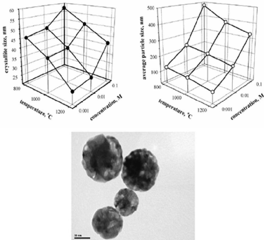
Fig. 18 Effect of furnace temperature during synthesis on the morphology and crystallinity of \text{BZrO}_3 nanopowders by USP (from M.M. Bucko & J. Obłakowski, J Eur Ceram Soc. , (2007) [Ref. 209])
