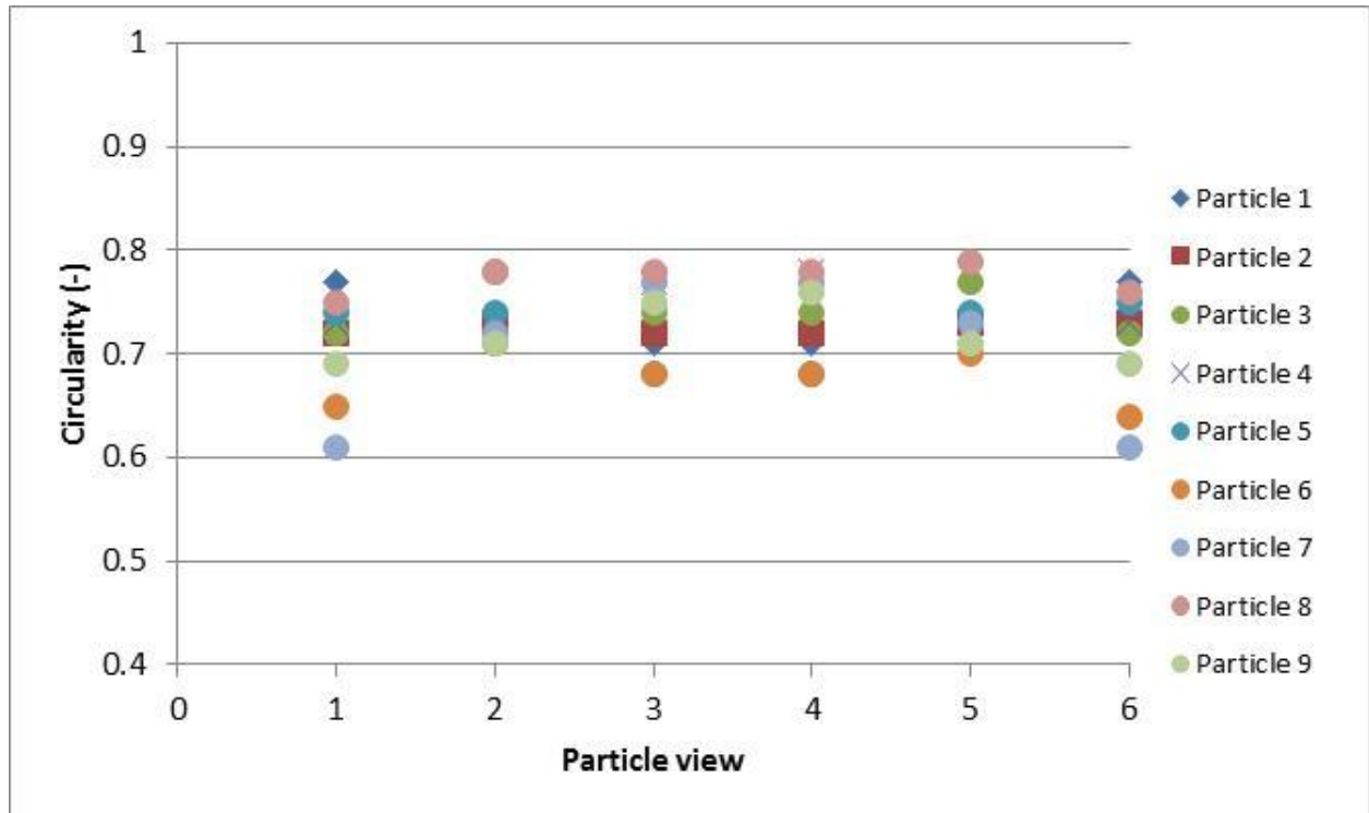
Figure 6: Circularity for the individual particle views
