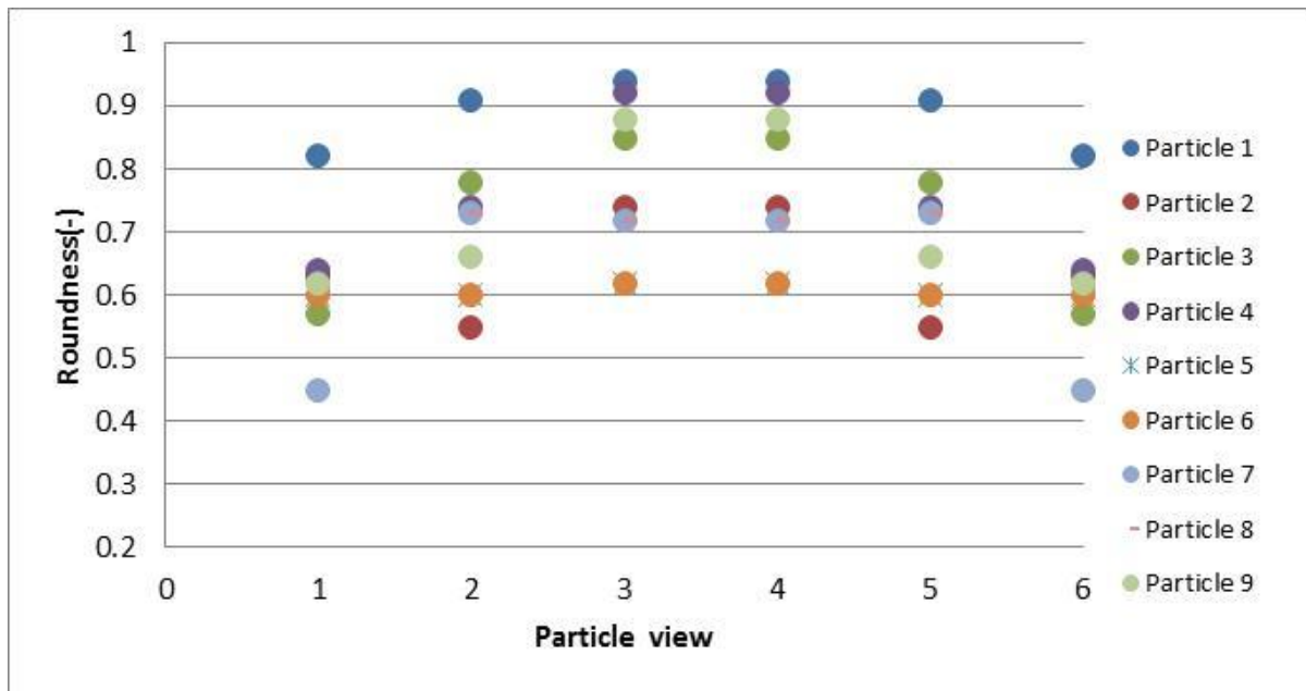
Figure 5: Roundness for the individual particle views
