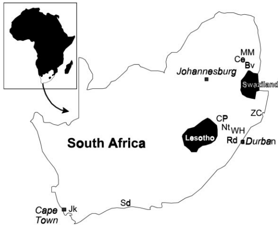
Fig. 1. The locations of the sites in South Africa from which soils were sampled for repellency testing. The location codes are used in Table 1 and the text.
